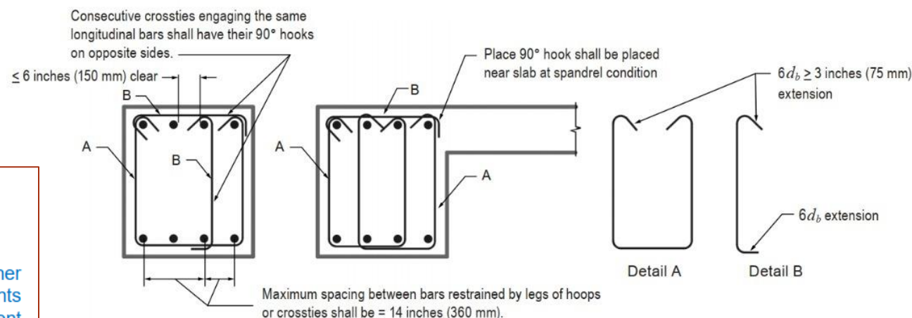
Figure 5-14. Hoop reinforcement detail.
